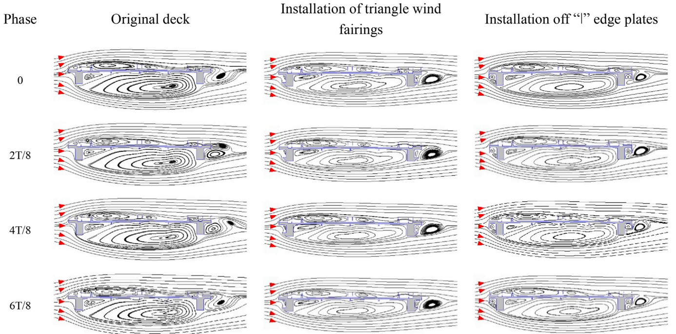
Fig. 16. Numerical simulation of improved bridge deck at 0^\circ attack angle.
